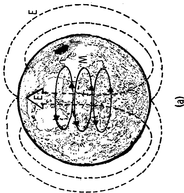
MAGNETIC FIELD OF MOON (M) GENERATED BY THE ELECTRIC FIELD E CARRIED IN THE SOLAR WIND
