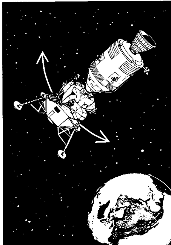
YAW-ROLL MANEUVER
