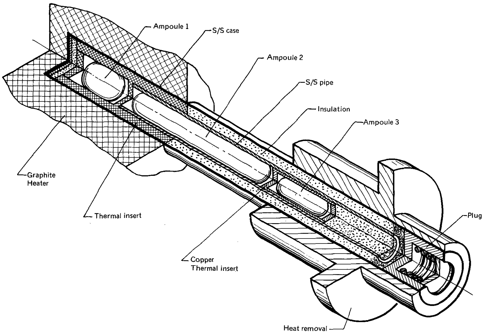
FIGURE 5.3 MULTIPURPOSE FURNACE EXPERIMENT CARTRIDGE
