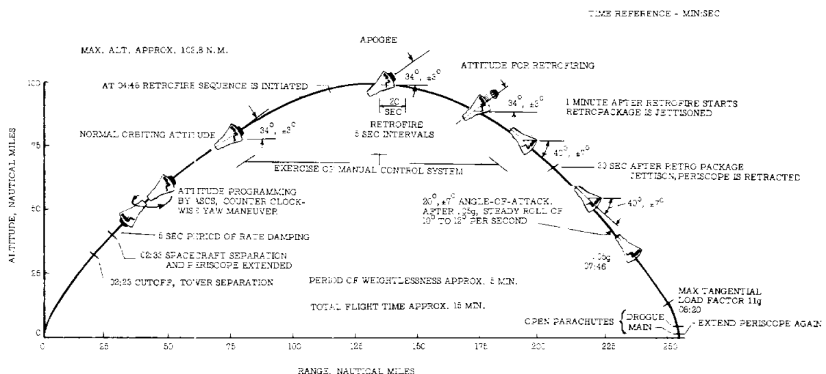
FIGURE 7-2. Mission profile.
