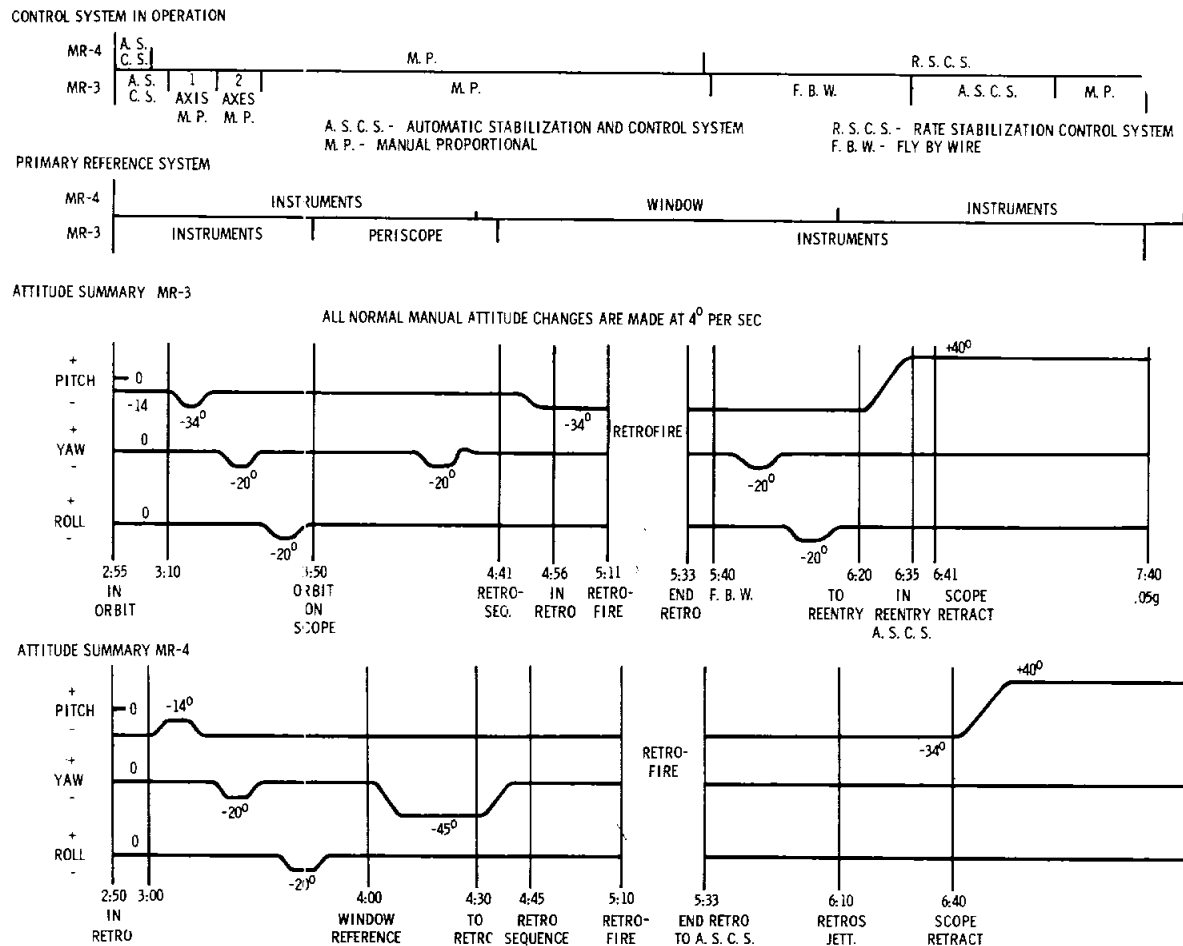
FIGURE 6-1. Manual control summary for the MR-3 and MR-4 flights.
