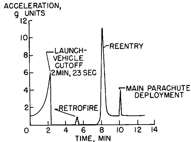
FIGURE 2-6. Acceleration time history for MR-4 flight.
