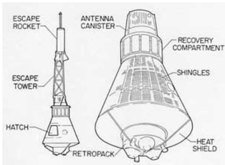
Figure 13. Spacecraft and escape system configuration.
