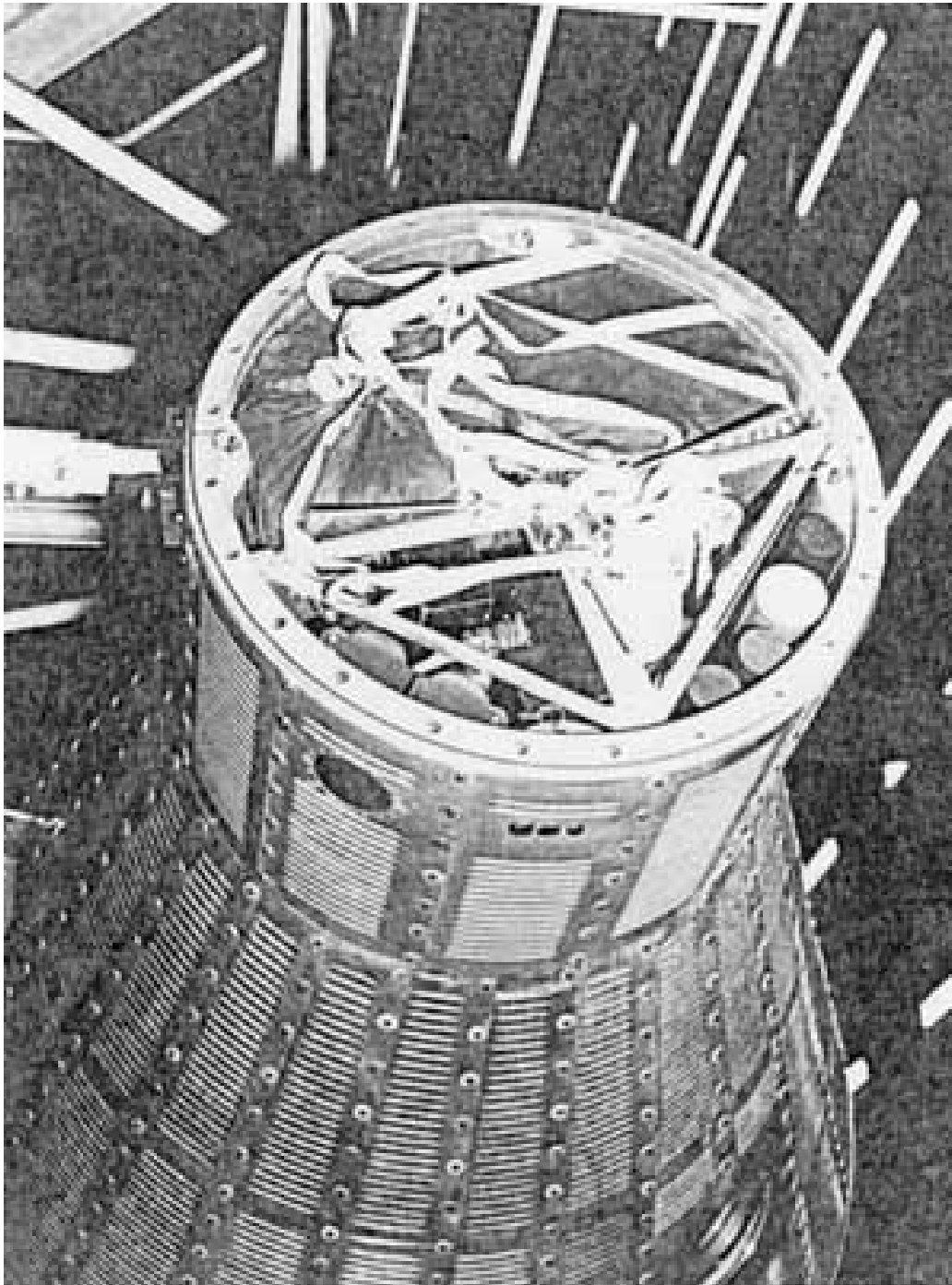
Figure 7. Equipment installation in the parachute canister.
