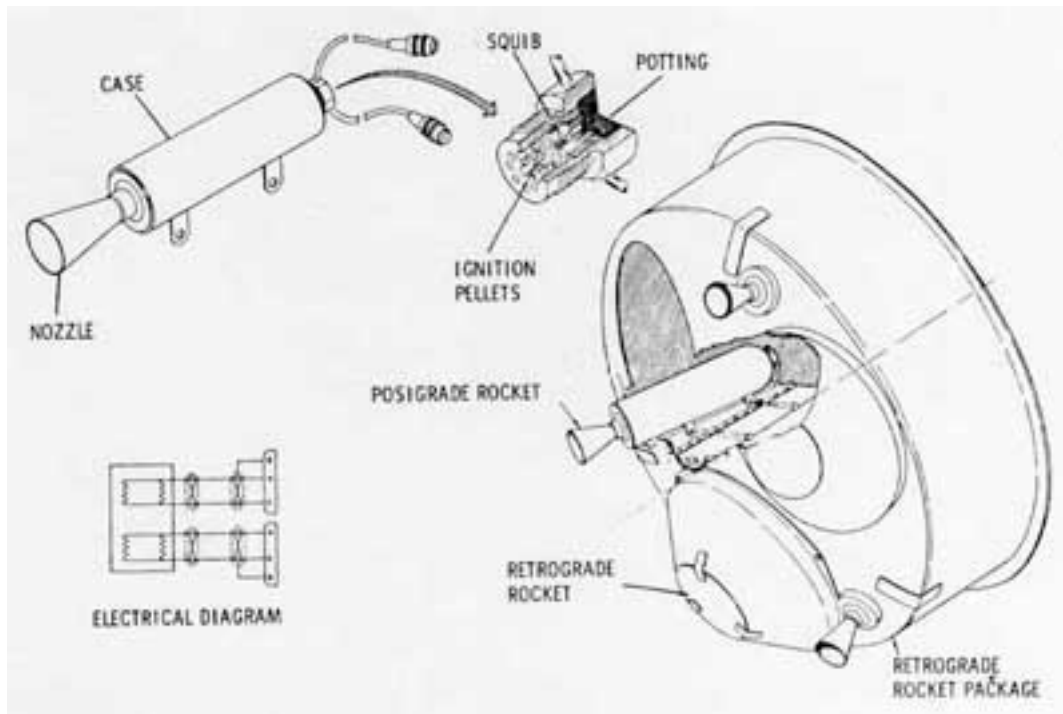
Figure 36. Posigrade rocket motors.
