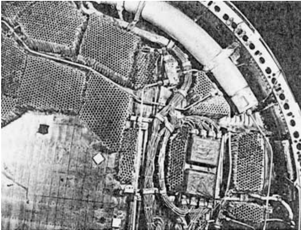
Figure 12. Honeycomb structure partially to absorb impact force.
