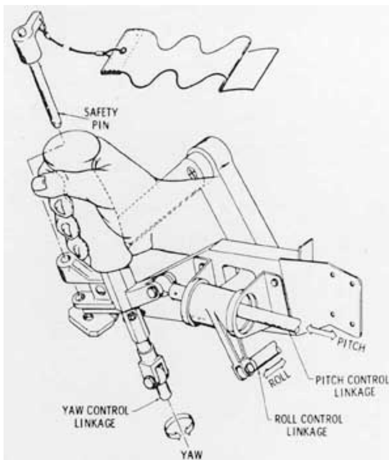
Figure 26. Three-axis hand controller.
