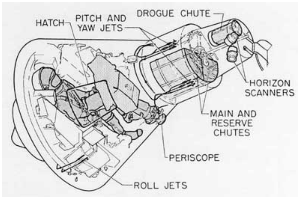
Figure 15. Spacecraft interior arrangement.
