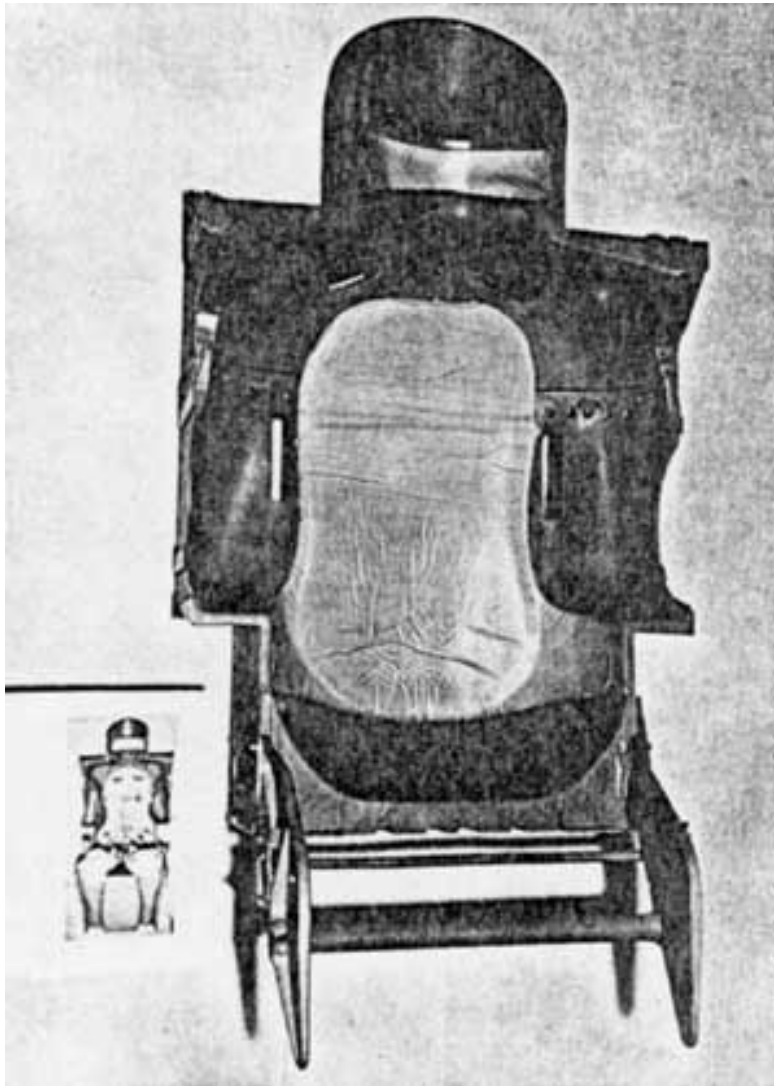
Figure 63. Astronaut couch modifications.
