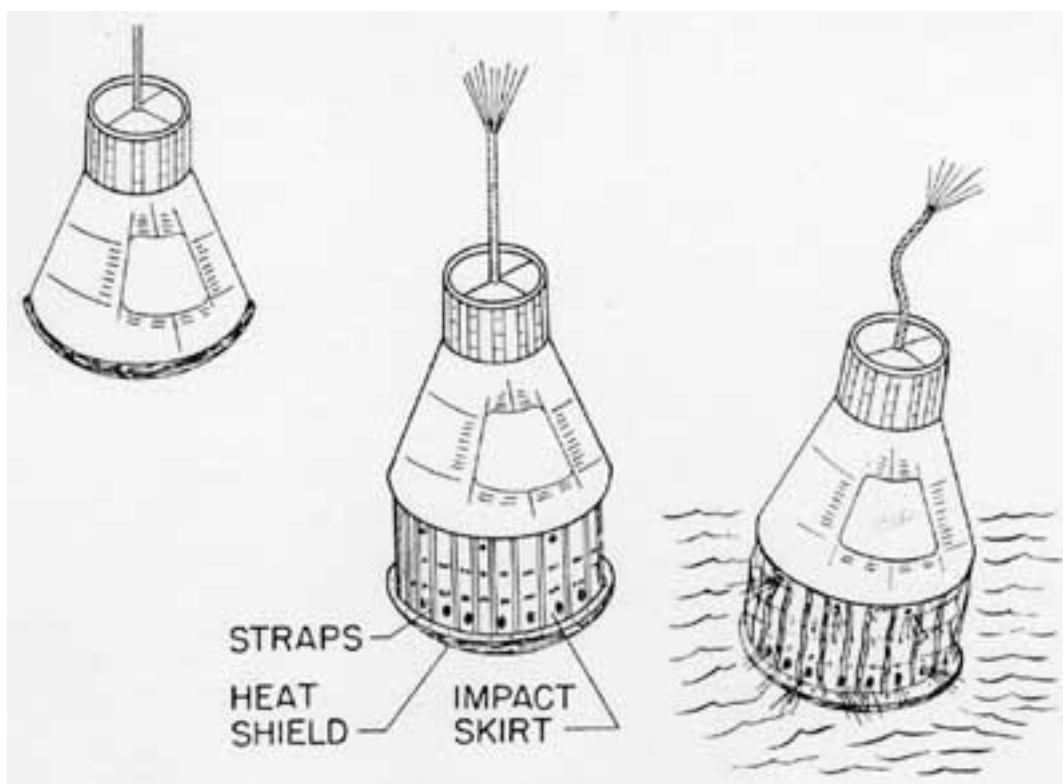
Figure 46. Impact attenuation.
