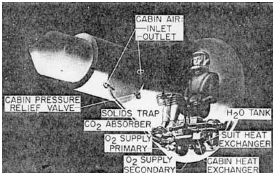
Figure 38. Mercury environmental control system.
