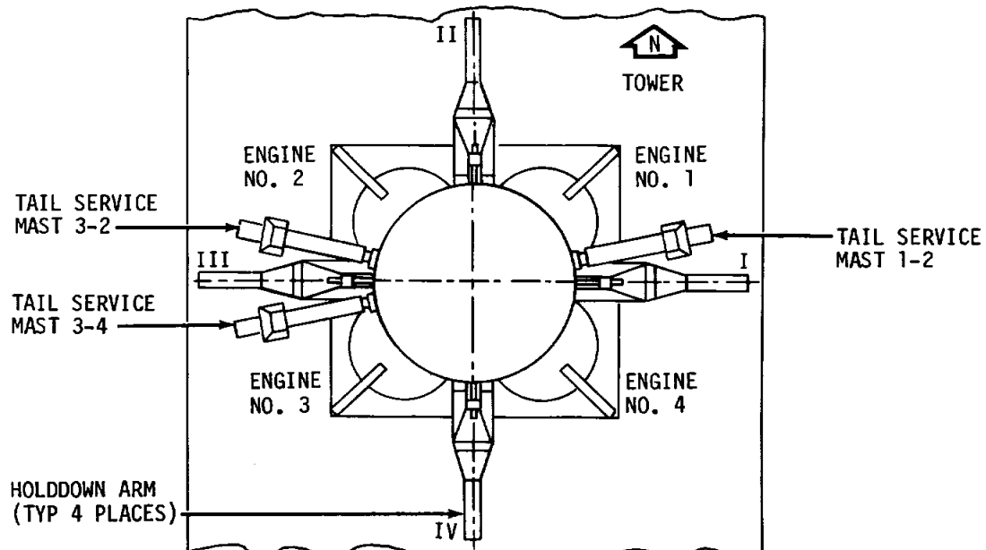
ENGINE/HOLDDOWN ARM/TAIL SERVICE MAST ORIENTATION
