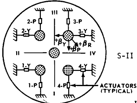
S-IC & S-II ACTUATOR LAYOUTS
