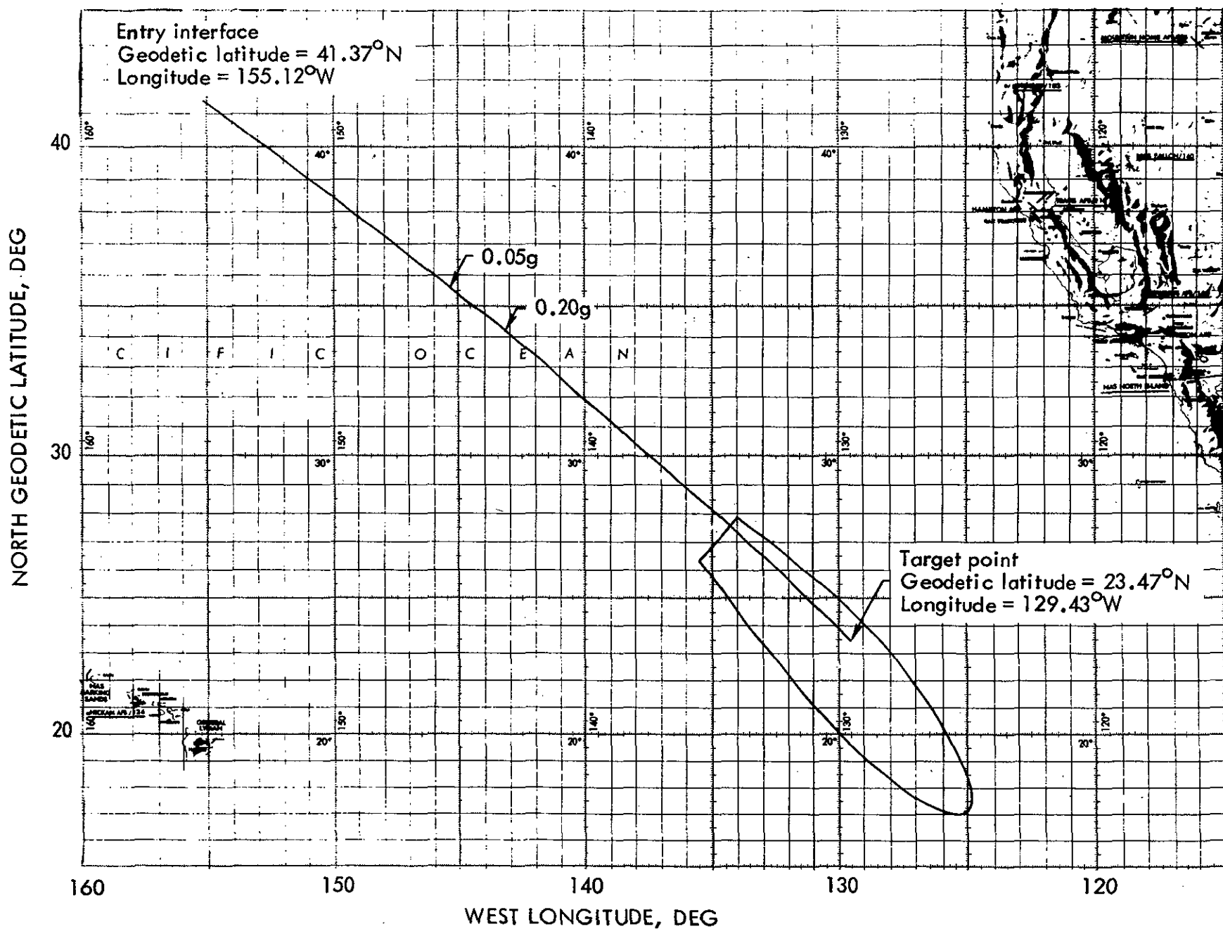
CM reentry track and maneuver envelope SW of NAS North Island, San Diego
