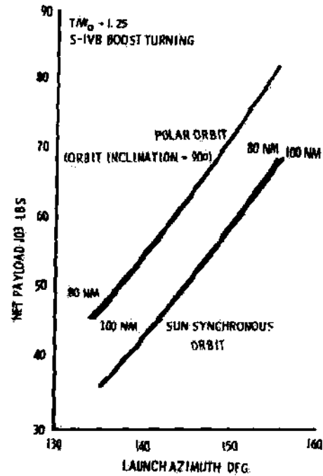
FIGURE 4-6 INT-20 POLAR & SUN SYNCHRONOUS PAYLOAD CAPABILITY (DIRECT ASCENT)
