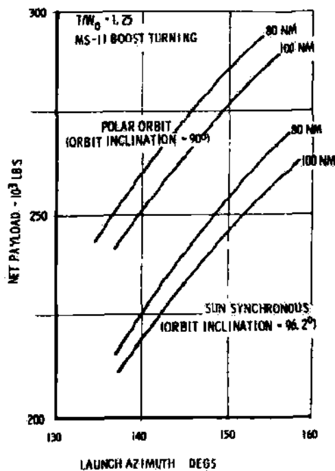
FIGURE 5-8 TWO-STAGE POLAR & SUN SYNCHRONOUS ORBIT PAYLOAD CAPABILITY
