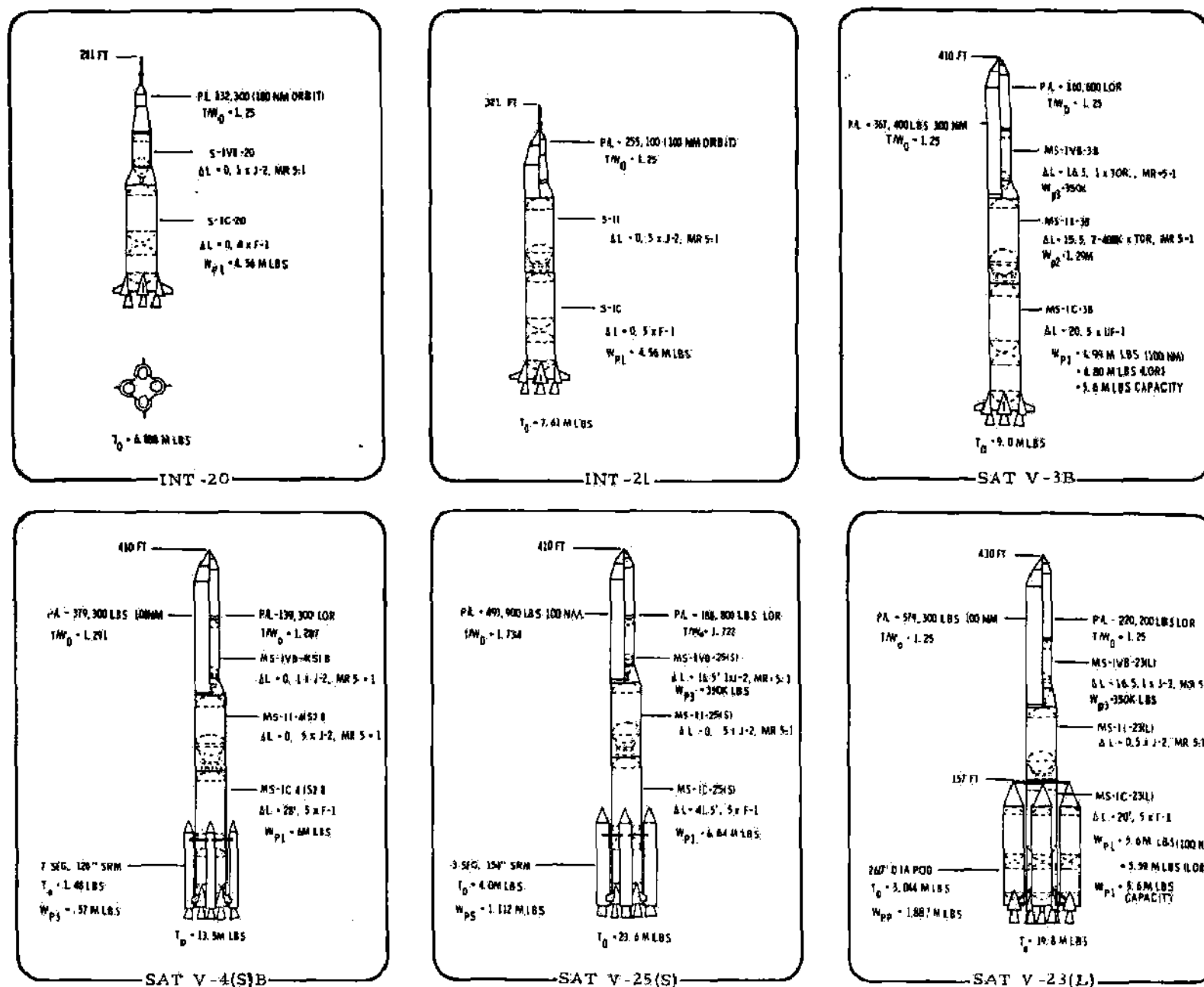
FIGURE 1-2 SELECTED BASELINE LAUNCH VEHICLES FOR PHASE II STUDY EFFORT
